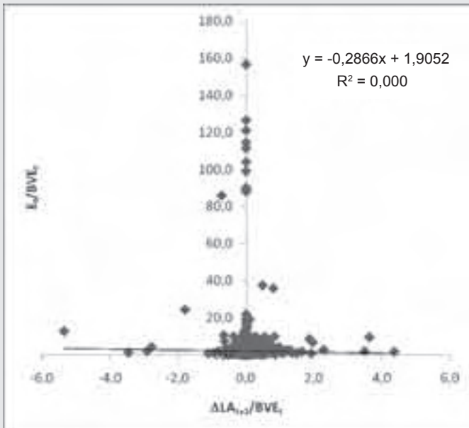
Dispersion Diagram for \Delta LA_{t+1} and E_t / BVE_t
