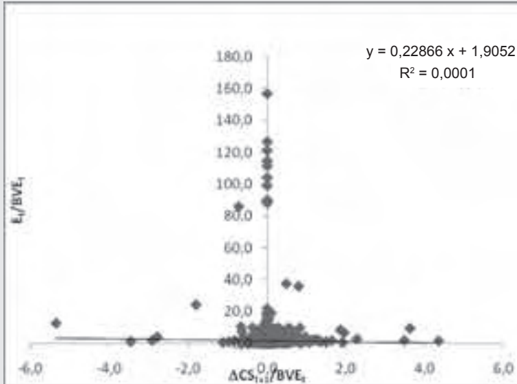
Dispersion Diagram for \Delta CS_{t+1} and E_t / BVE_t
